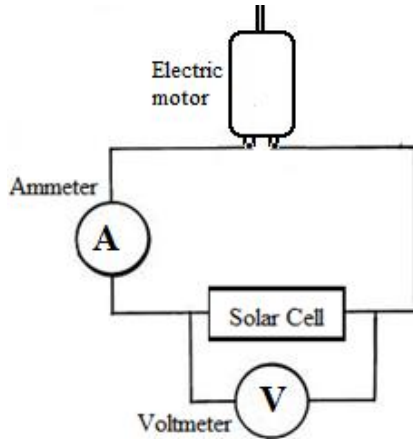
(a) Figure 2: (a) Solar cell efficiency test circuit diagram (b) Experimental set up
